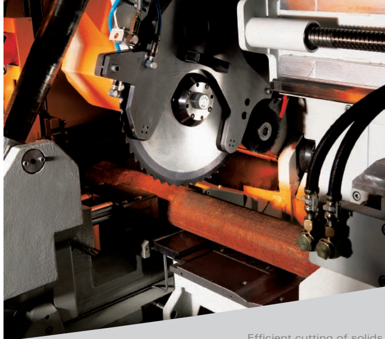
Efficient cutting of solids, profiles and tubes of all material qualities, even difficult to cut grades
