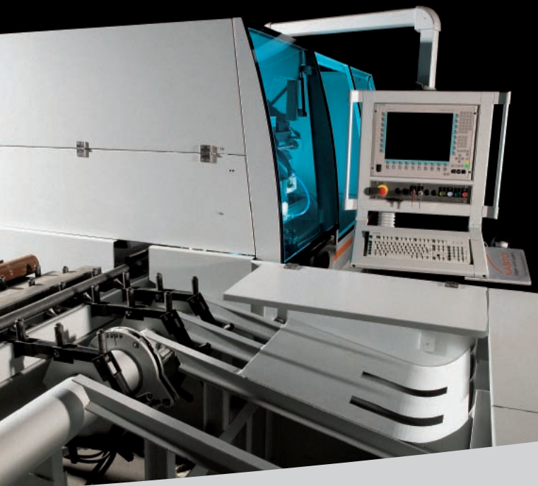
KASTO TechnoControl : Easy shop-oriented operation with menu control via function keys.
